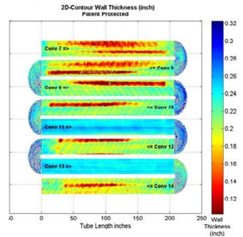
Figure 3. Wall thinning as seen in Quest Integrity data
