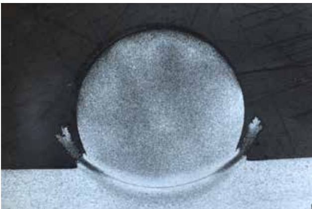
Weld spatter damage on parent material
