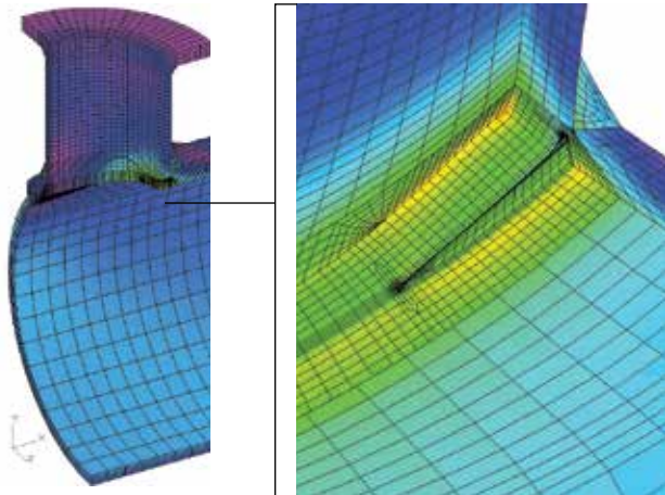
Pressure vessel with a surface crack located at the internal weld of a nozzle.
