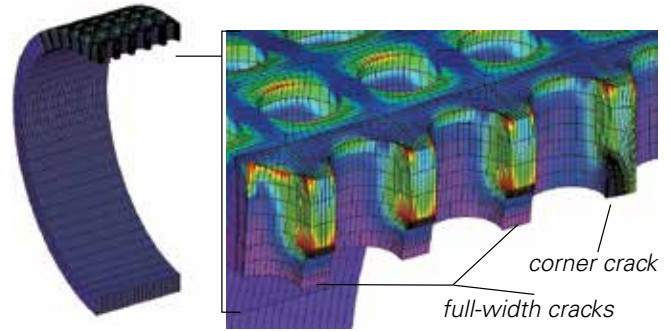
Cracked ligaments along generating bank tube holes in an electric power steam drum.
