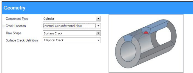
Extensive Library of Structural Geometries and Crack Shapes
