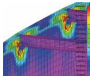
Stress analysis of a fixed roof connection
