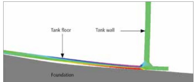
Floor settlement stress results on an axisymmetric model
