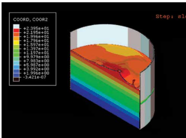
Dynamic analysis of tank subject to earthquake loads
