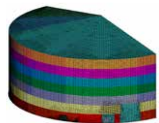
1/2 symmetric model of storage tank with repairs
