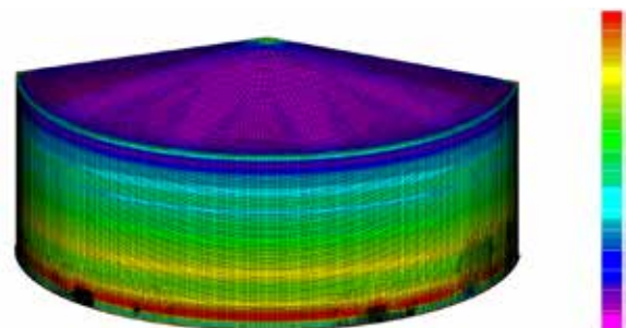
Hoop stress due to hydrostatic pressure
